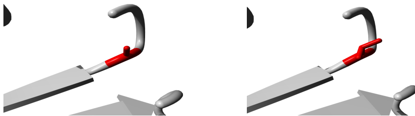
Figure 2.13: Molecular visualization of the WT (left) and variant (right) amino acid. The residues colored in red represents the wild type (ALA) and variant residue (THR).
